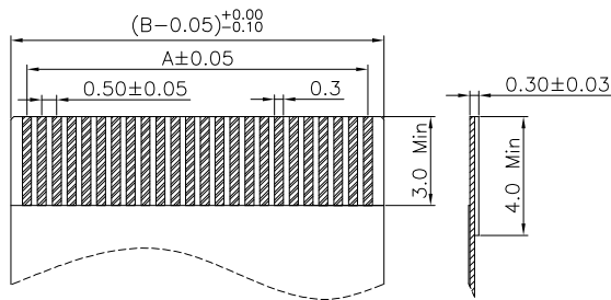
适用编平线 (Applicable Flat Cable)
